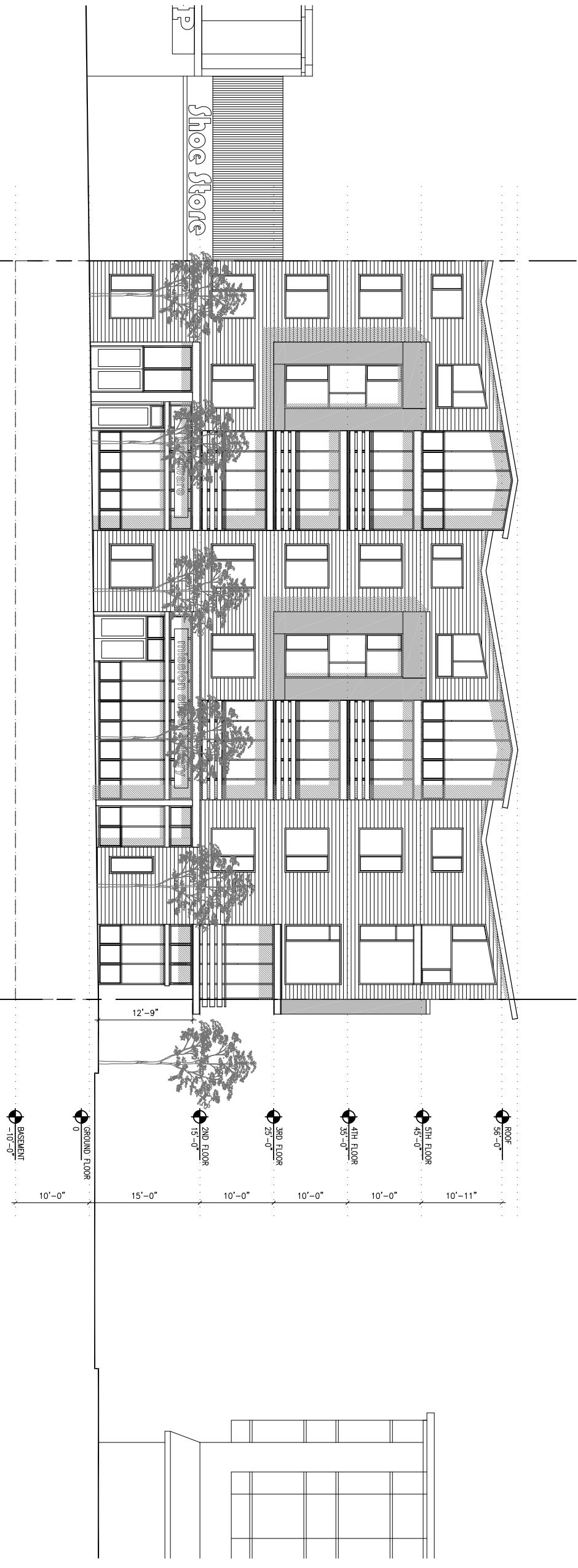
1 MISSION STREET / NORTH ELEVATION 56'
